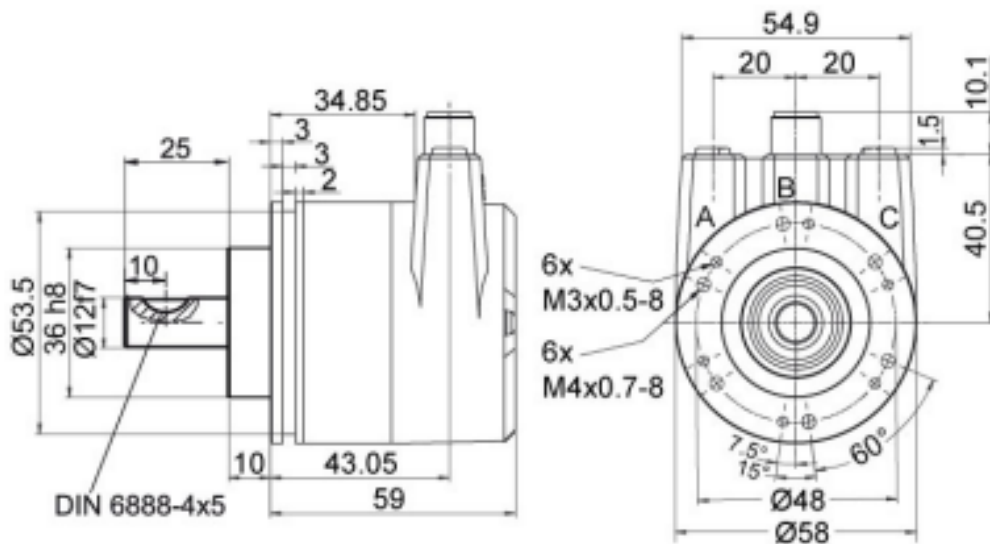
Figure 5.3: Dimensions WDGA 58D
